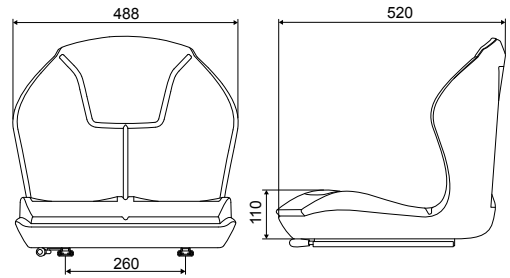
Universal seat pan with slide rails
